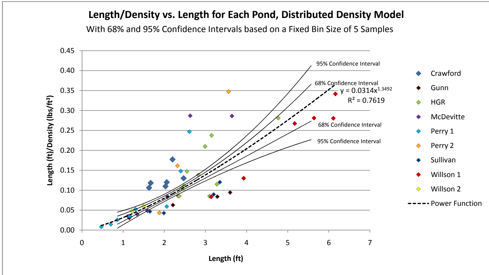
FIGURE 31 - Regression analysis of normalized density for pond cores showing the relationship of each pond-specific core's distribution to the overall bulk density distribution
