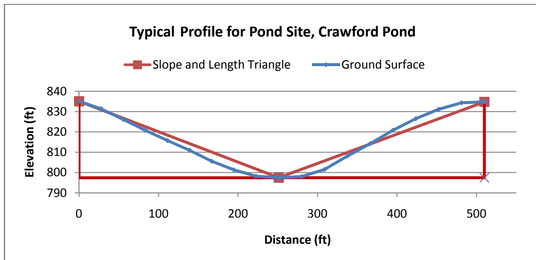
FIGURE 30 - Valley cross section with representative slopes and lengths
