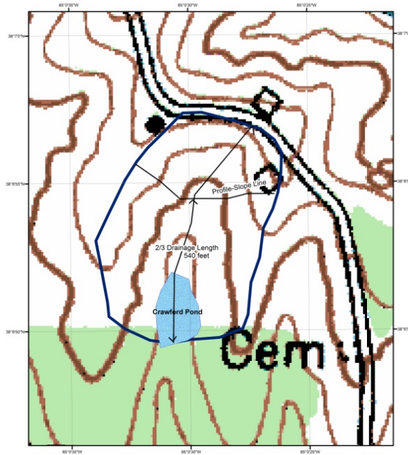
Crawford Pond Detail: Hill Slope and Length for RUSLE2
