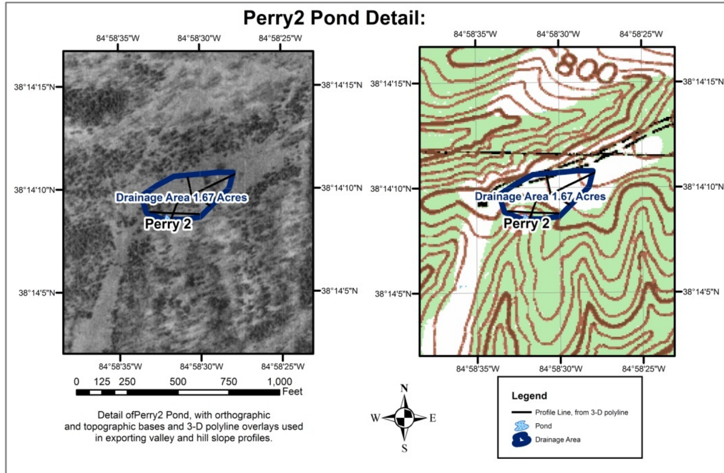
FIGURE 56 - Orthographic and topographic layout of Perry2 pond site.
